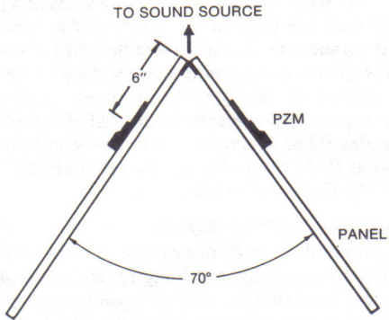
PANEL ARRANGEMENT FOR ORTF STEREO
